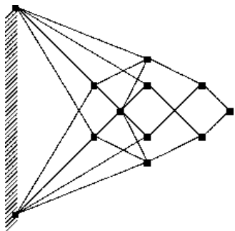
Robust Design: Dream and Reality The compliance w.r.t. f^n is 1.0024
