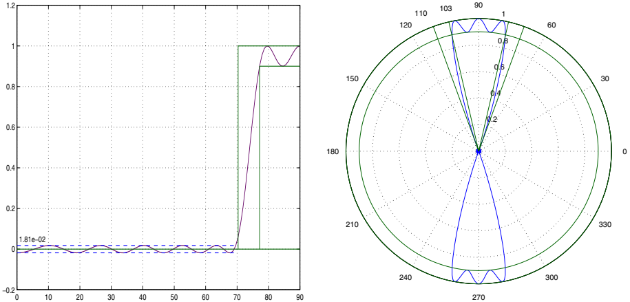
Dream: Nominal design, no implementation errors Sidelobe attenuation level 0.018 (left diagram is in polar coordinates)
